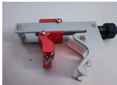
Tools for chamfering primary insulation
