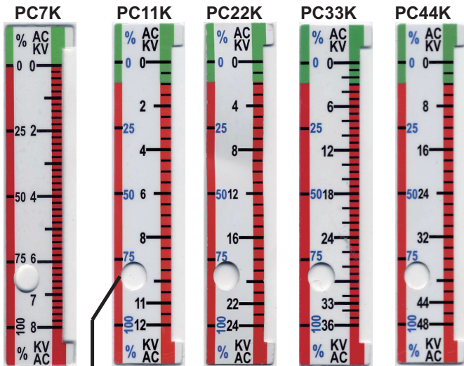
Neon Indicator
